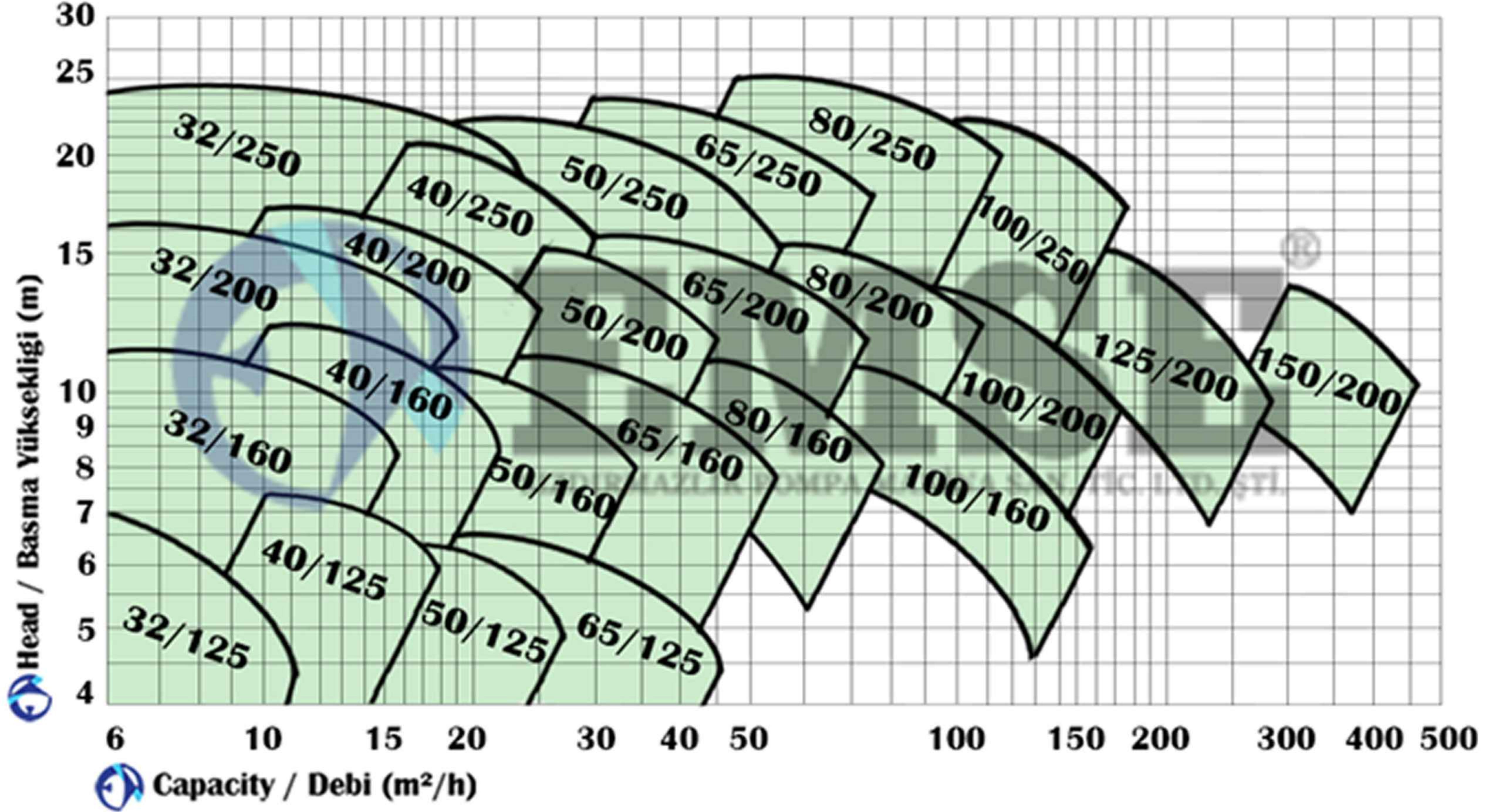
1450 RPM 50HZ CURVE
