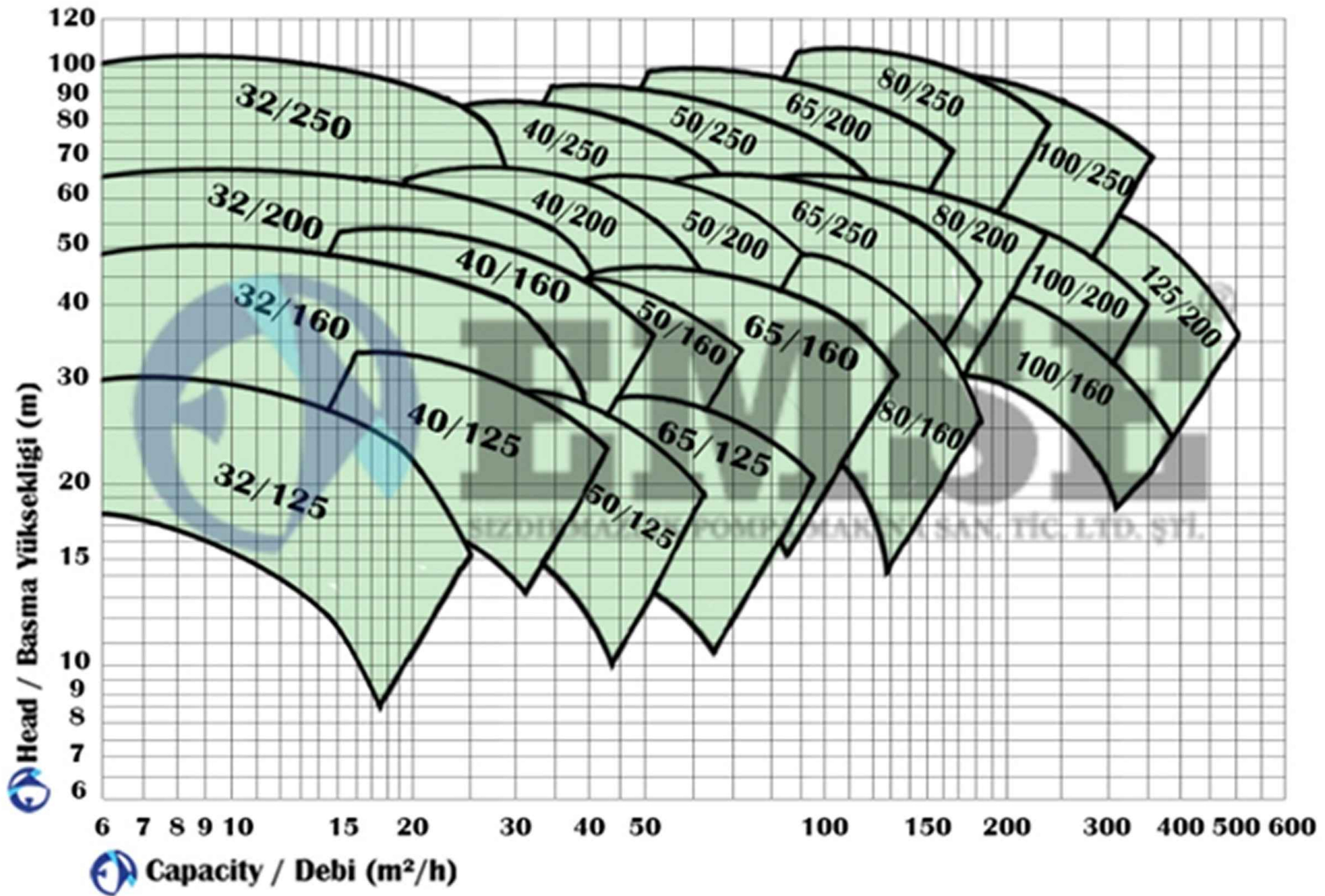
2900 RPM 50HZ CURVE
