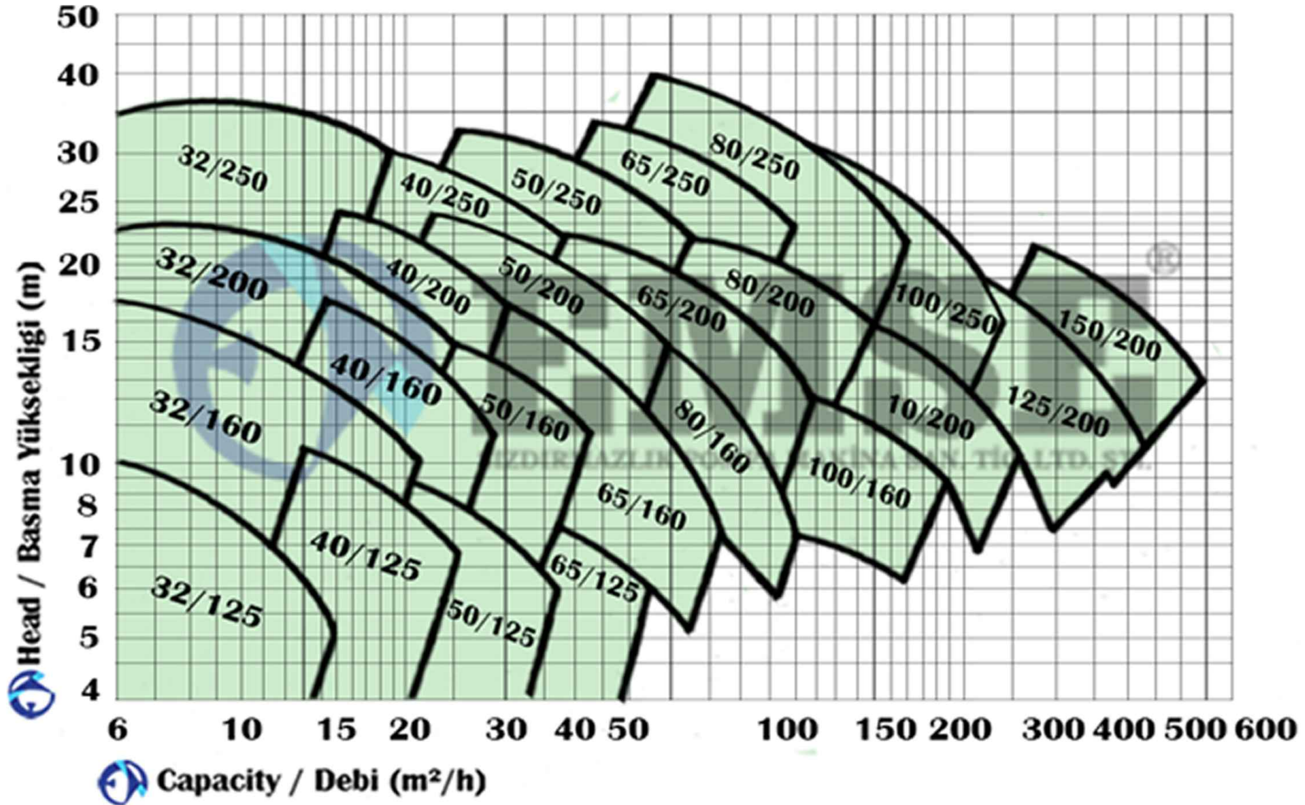
1750 RPM 60HZ CURVE
