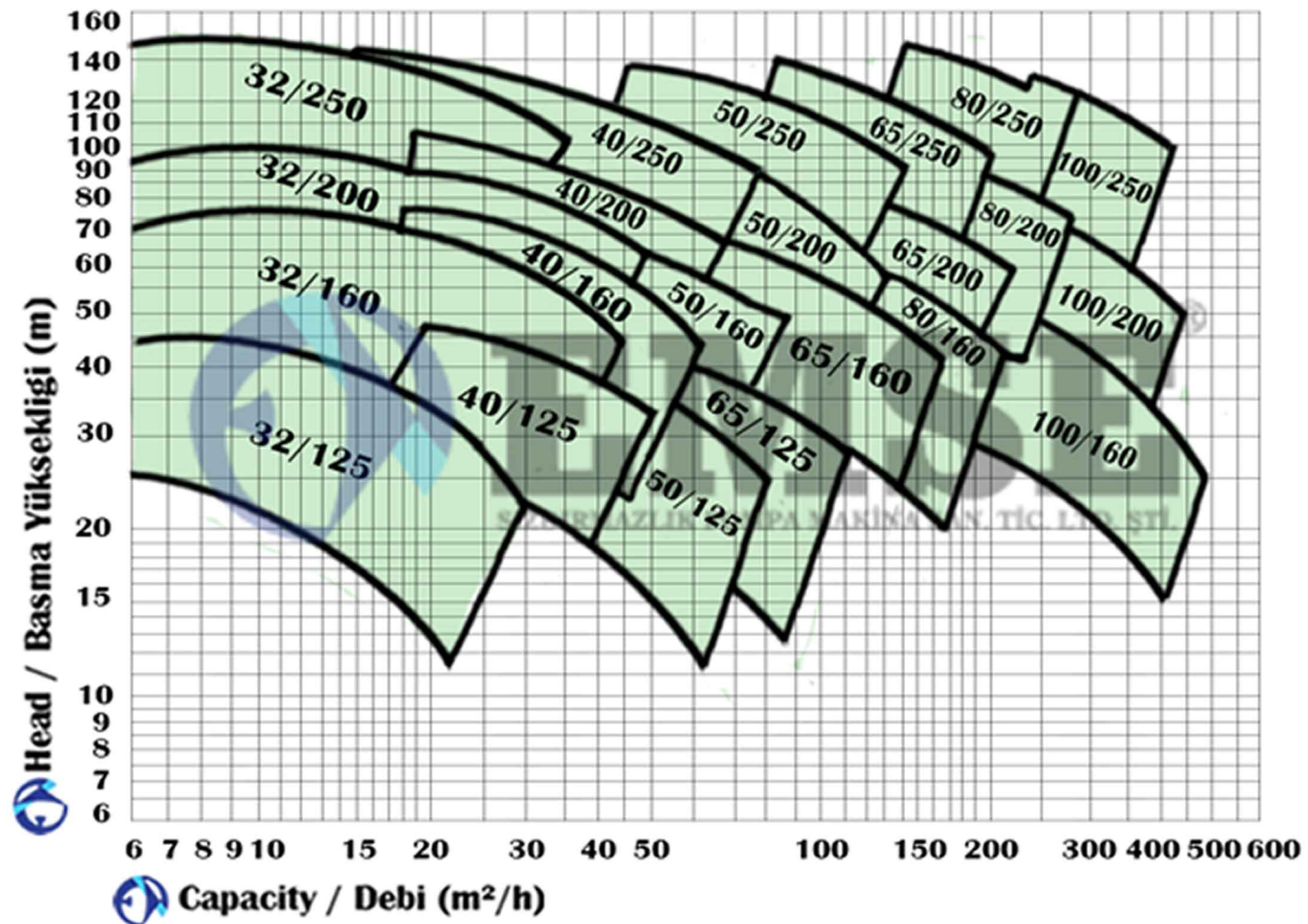
3500 RPM 60HZ CURVE
